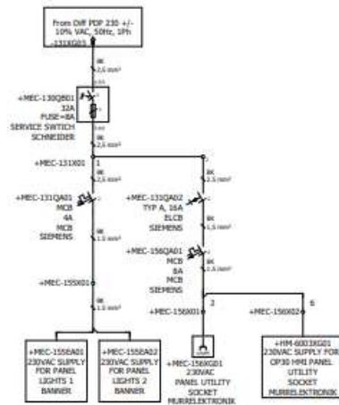
SINGLE LINE DIAGRAM POWER ARCHITECTURE
